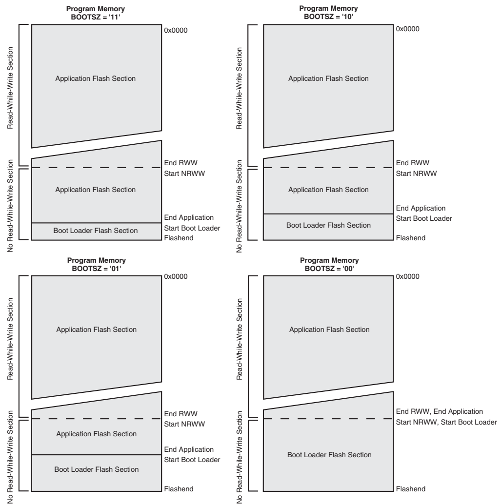
Figure 24-2. Memory Sections
